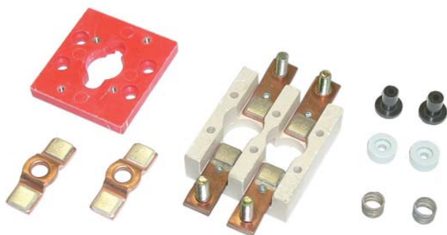
Type: HB437KP Tip size: 9,5 X 9,5 mm
