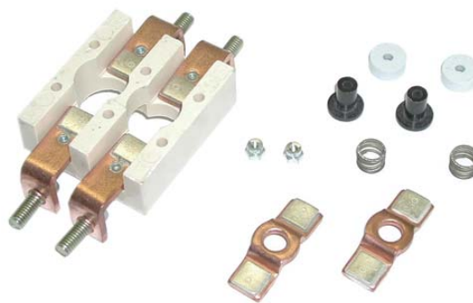
Type: HB437K Tip size: 9,5 X 9,5 mm
