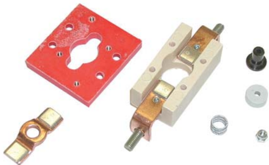
Type: HB431-CAT Tip size: 9,5 X 9,5 mm
