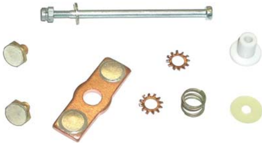
Type: HBSP102 Tip size: Ø 9,5 mm
