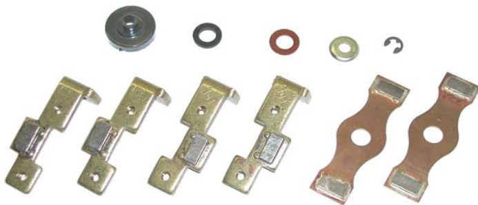
Type: I23100 Tip size: 5,9 X 12 mm
