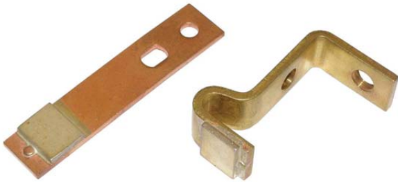
Type: MEIDEN - MZ2 Tip size: 12 X 15 mm
